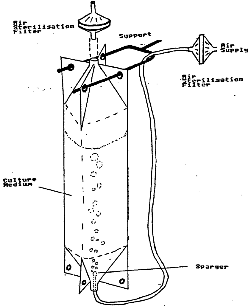
FIGURE 1 SMALL FERMENTER
